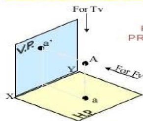
POINT A ABOVE HP & IN FRONT OF VP
