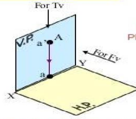
POINT A ABOVE HP & IN VP
